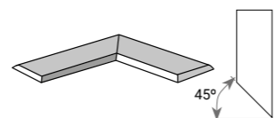
BORDE ÁNGULO EXTERIOR RE STAIR TREAD COPING TILE (OUTER CORNER)
